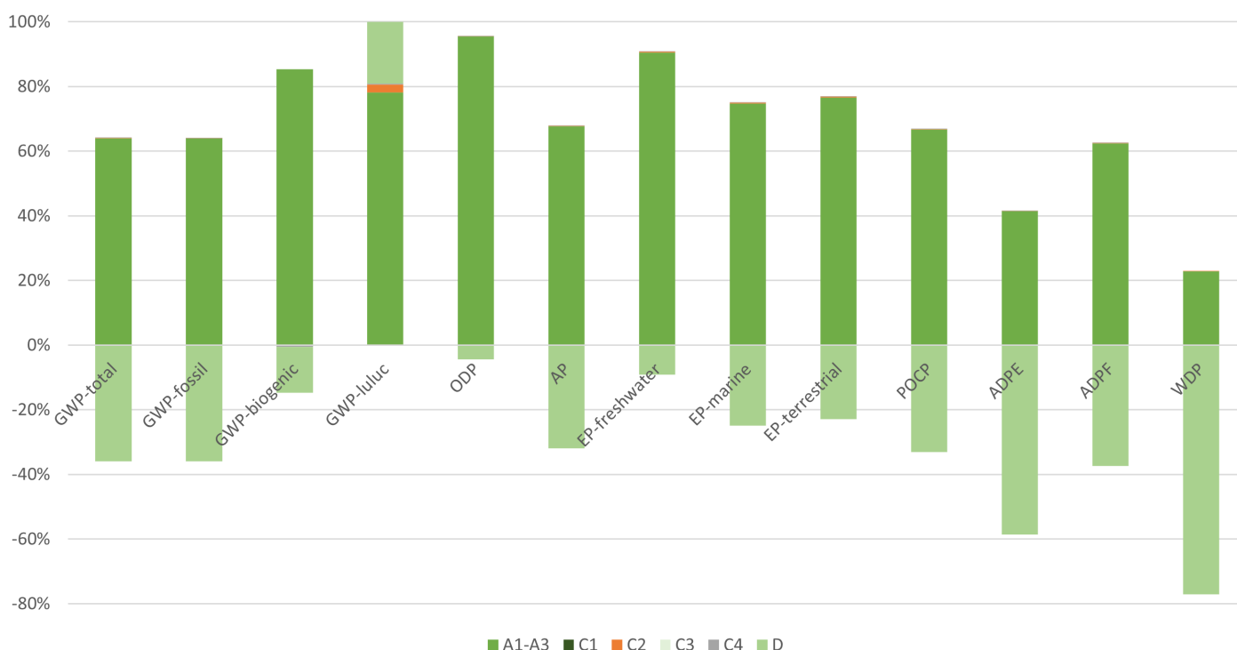
Hot-spot analysis of voestalpine heavy plates
